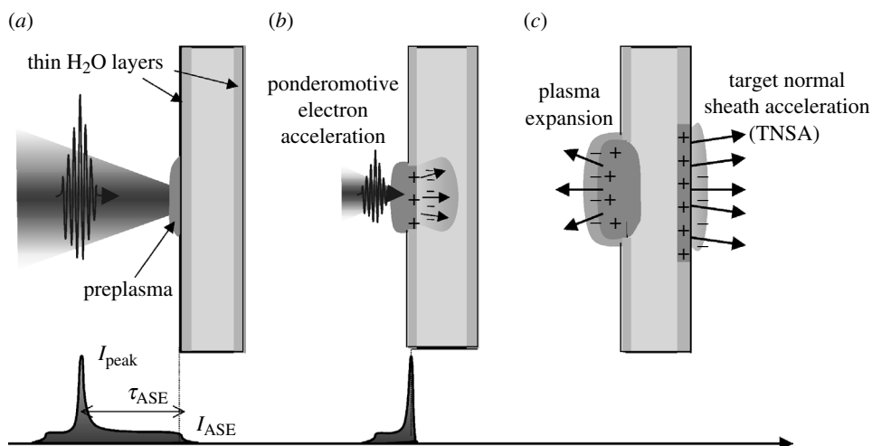
Figure 1. The main ion acceleration mechanisms in the interaction of a high-intensity laser pulse with a thin foil target. (a) The ASE-pedestal arriving at the target surface, prior to the peak of the laser pulse, creates a plasma. (b) The peak intensity of the laser pulse interacts with the preformed plasma, ponderomotively accelerating electrons into the target and creating a space charge separation, leading to ion acceleration. (c) The accelerated electrons emerge from the target rear surface, forming an electron sheath with micron-scale Debye length. The resulting quasi-static electric field, of the order of \text{TV m}^{-1} , leads to ionization and ion acceleration to multi-MeV energies (the TNSA mechanism). Plasma expansion at the target front surface leads to ion acceleration in the backward direction.
