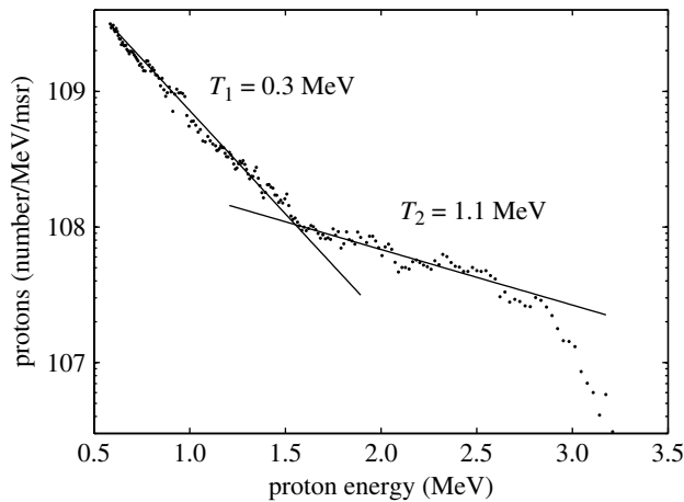
Figure 5. A typical proton energy spectrum, observed by irradiating a 6 μm thick Al foil at a few 10^{19} W cm ^{-2} . The spectrum comprises of two Boltzmann-like distributions with temperatures of 0.3 and 1.1 MeV.
