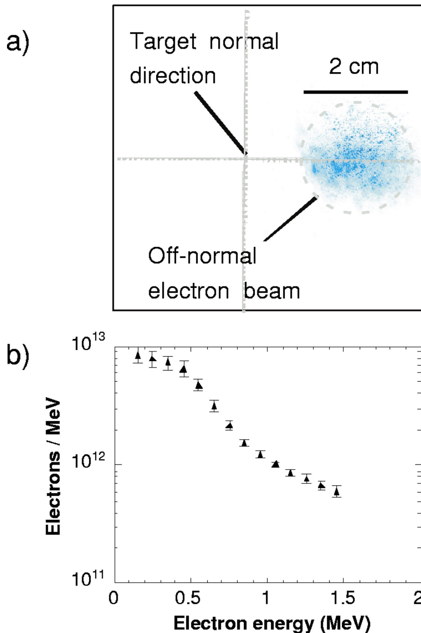
FIG. 2. (Color) Off-normal filamentary electron beam from two laser beam experiments. (a) is a typical electron filamented beam recorded on a RCF layer at the depth of 1240\ \mu\text{m} in the rear stack; (b) is the energy spectrum of the off-normal electron beam. The intensities of the main interaction beam and beam 2 (heating beam) are 10^{19}\ \text{W cm}^{-2} and 5 \times 10^{18}\ \text{W cm}^{-2} , respectively. The two beams were coincident in time.
