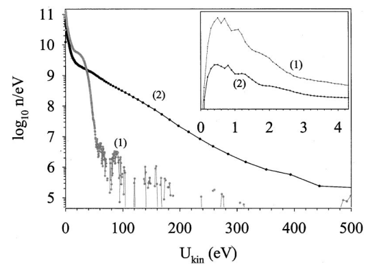
FIG. 2. Kinetic-energy distribution of photoelectrons from a silver film measured as a function of incident intensity. The inset shows the peak of electrons of low kinetic energies on a linear scale. The incident power densities are 12.5 GW/cm 2 (1) and 40 TW/cm 2 (2). The experimental data were averaged into 0.1 eV energy bins, resulting in an energy resolution ranging from 0.1 eV at low energy to 40 eV at 0.4 keV.
